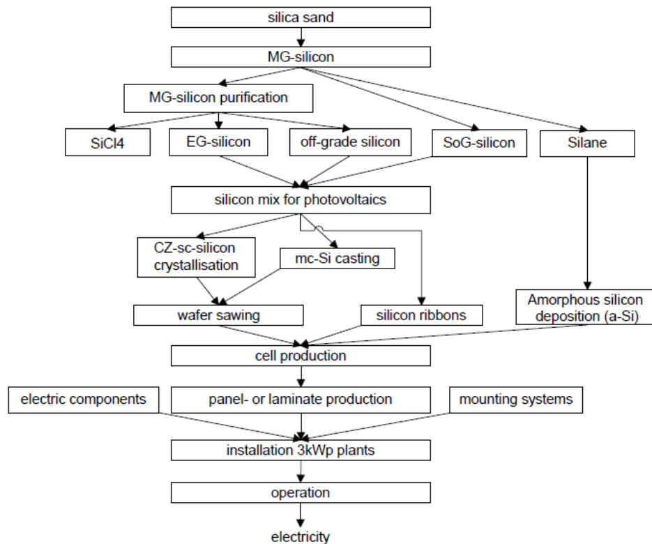
Figure 36: Subsystems for PV silicon based plants (Ecoinvent 2009).
