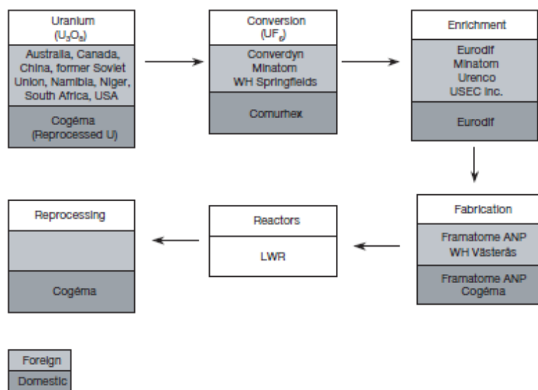
Figure 57: Material flow in the French nuclear fuel cycle (IAEA 2005).
