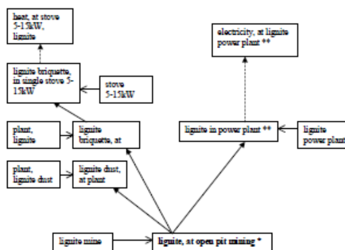
Fig. 6.1 Schematic picture of the modelled lignite chain.
